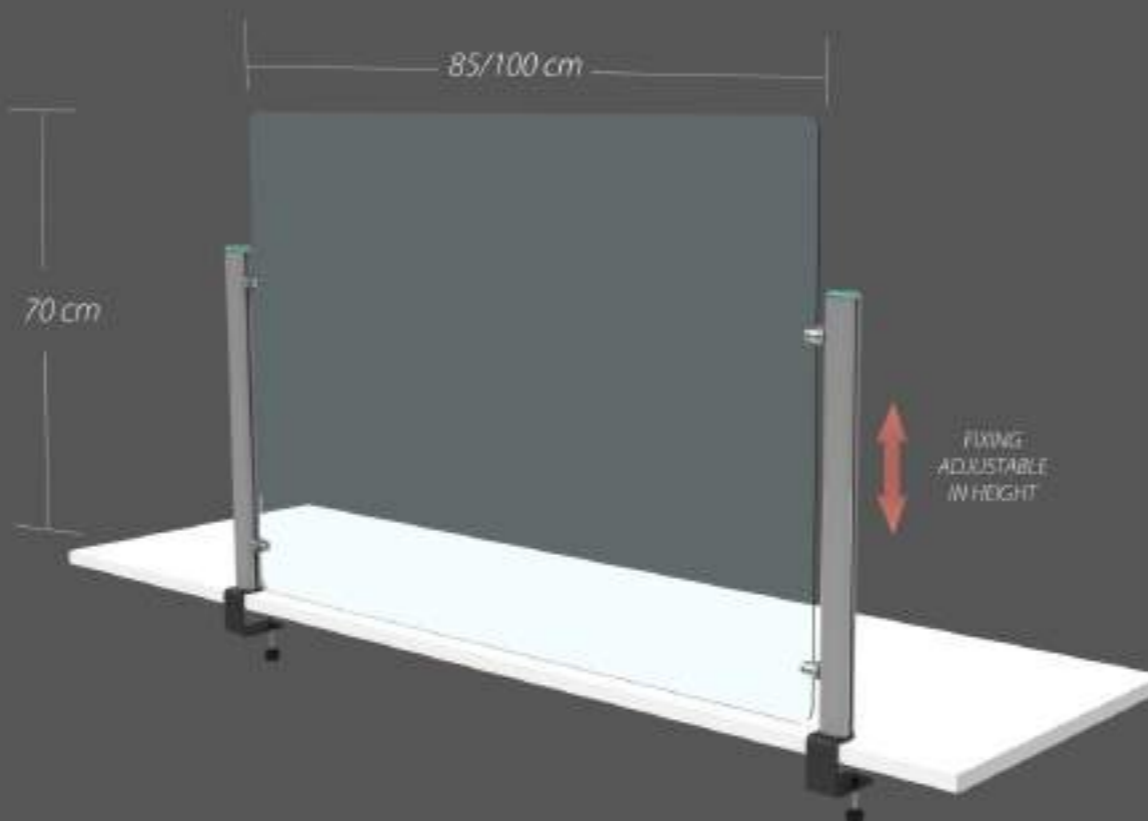
MATERIAL: TRANSPARENT METHACRYLATE, ALUMINIUM PROFILE AND CLAMPS
