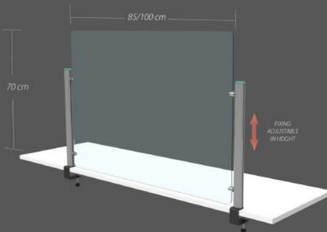
MATERIAL: TRANSPARENT METHACRYLATE, ALLUMINIUM PROFILE AND CLAMPS
